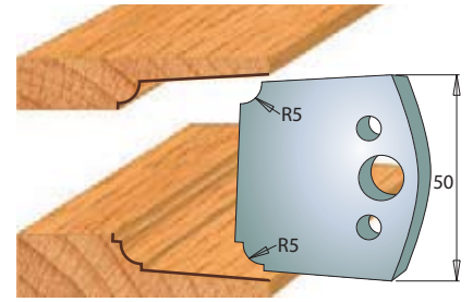
Pair of knives 690.579 Pair of limiters 691.579
